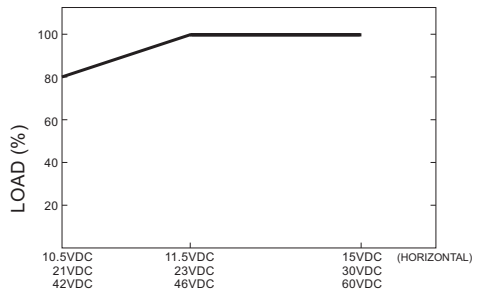
Figure 7.3 Input Derating Curve
