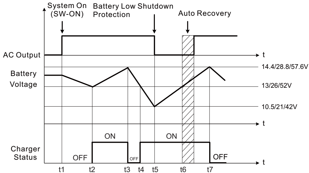
Figure 5.1 Operation Sequence
