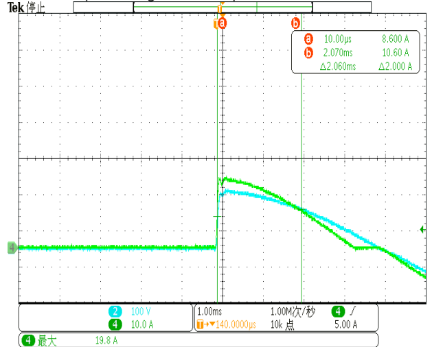
INPUT=115VAC/ 60HZ @ FULL LOAD
