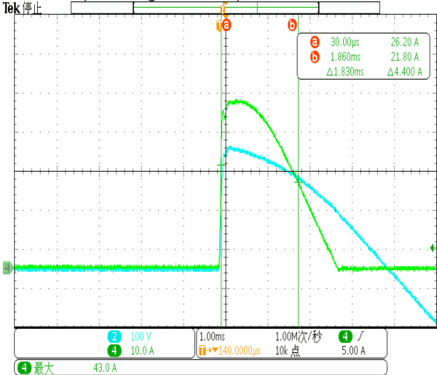
INPUT=230VAC/50HZ @ FULL LOAD
